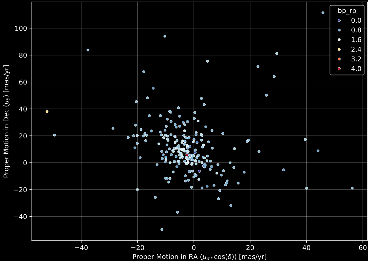
GALAH DR4 Field: [7170] Proper Motion Diagram (n= 229)
